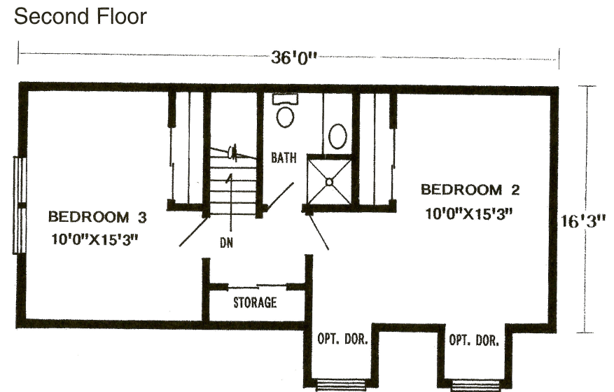
SUGGESTED OPTIONAL SECOND FLOOR PLAN
