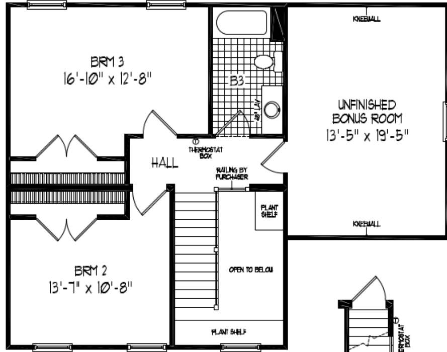
2ND LEVEL
